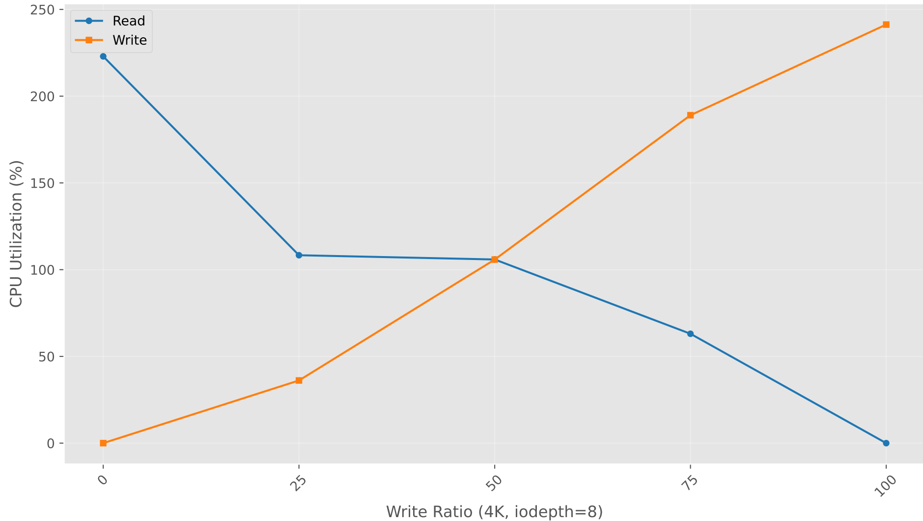
CPU Total vs Write Ratio (4K, iodepth=8)
